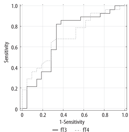
FIGURE 5. ROC curves for ft3 and ft4. ICU survival rate. Suggested cut-off points: 1.8 and 10.5 for ft3 and ft4, respectively
